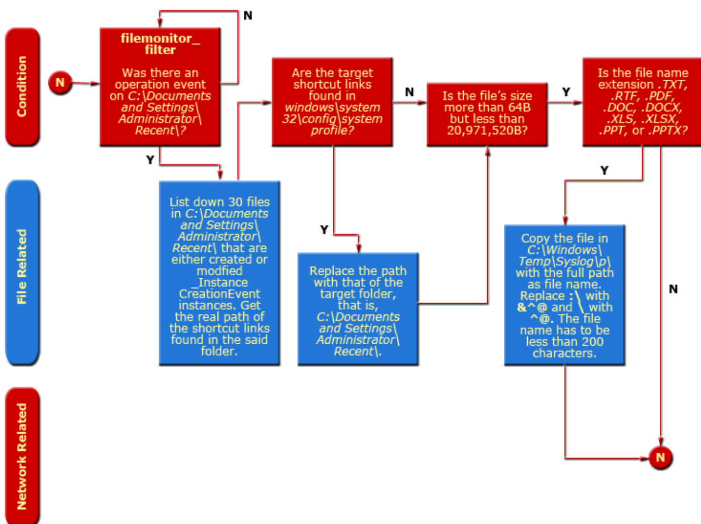
Figure 11. How TROJ_WMIGHOST.A uses the filemonitor_consumer script
