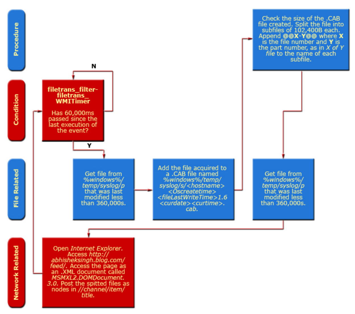
Figure 12. How TROJ_WMIGHOST.A uses the filetrans_consumer script
