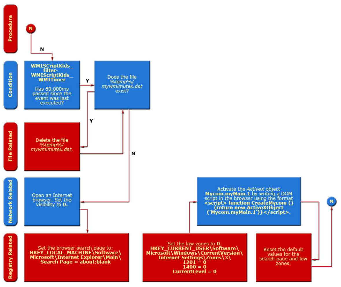
Figure 13. How TROJ_WMIGHOST.A uses the WMIScriptKids_consumer script
