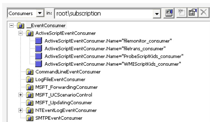
Figure 3. __EventConsumer class
