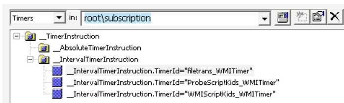
Figure 9. __TimerInstruction class
