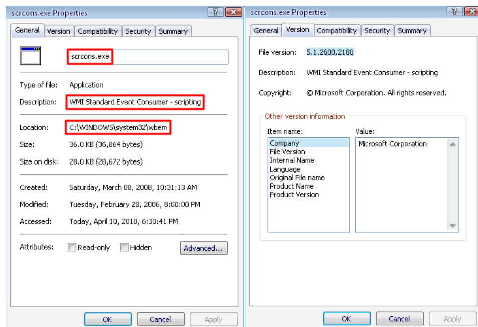
Figure 5. Srcons.exe's properties
